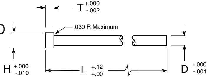
Standard Ejector Pins
